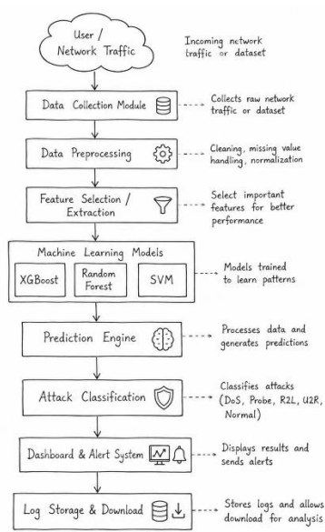
Fig. 1.1 System Architecture
