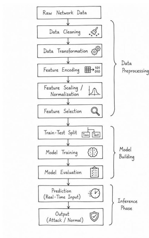
Fig. 1.2 Data Pipeline
